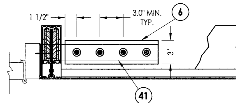
4 12 HORIZONTAL CROSS SECTION @ DOOR JAMB Sill & sill cover partially removed for clarity
