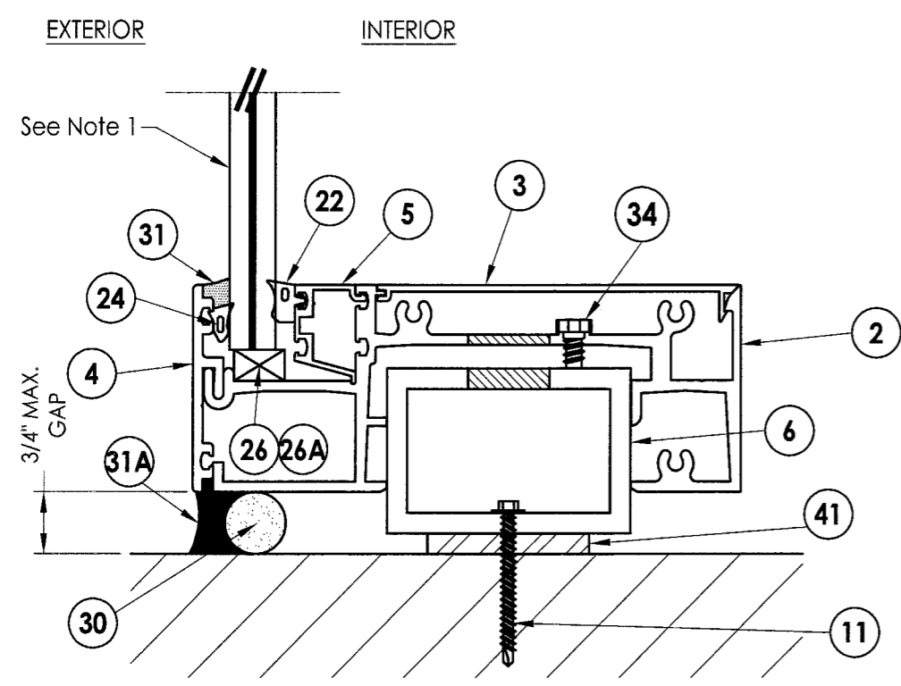
3 VERTICAL CROSS SECTION 7 Sill Detail w/ Steel Angle Clip Dry Glazed Option
