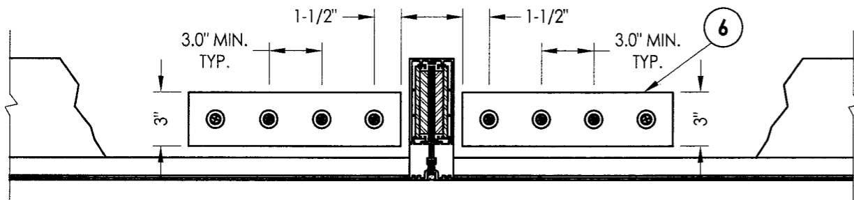
3 12 HORIZONTAL CROSS SECTION @ DOOR JAMB Head & head cover partially removed for clarity
