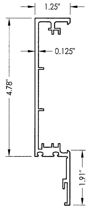
12 MULLION FEMALE
