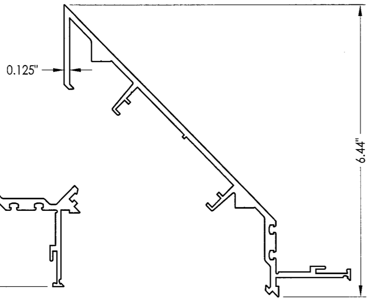
9 FEMALE CORNER
