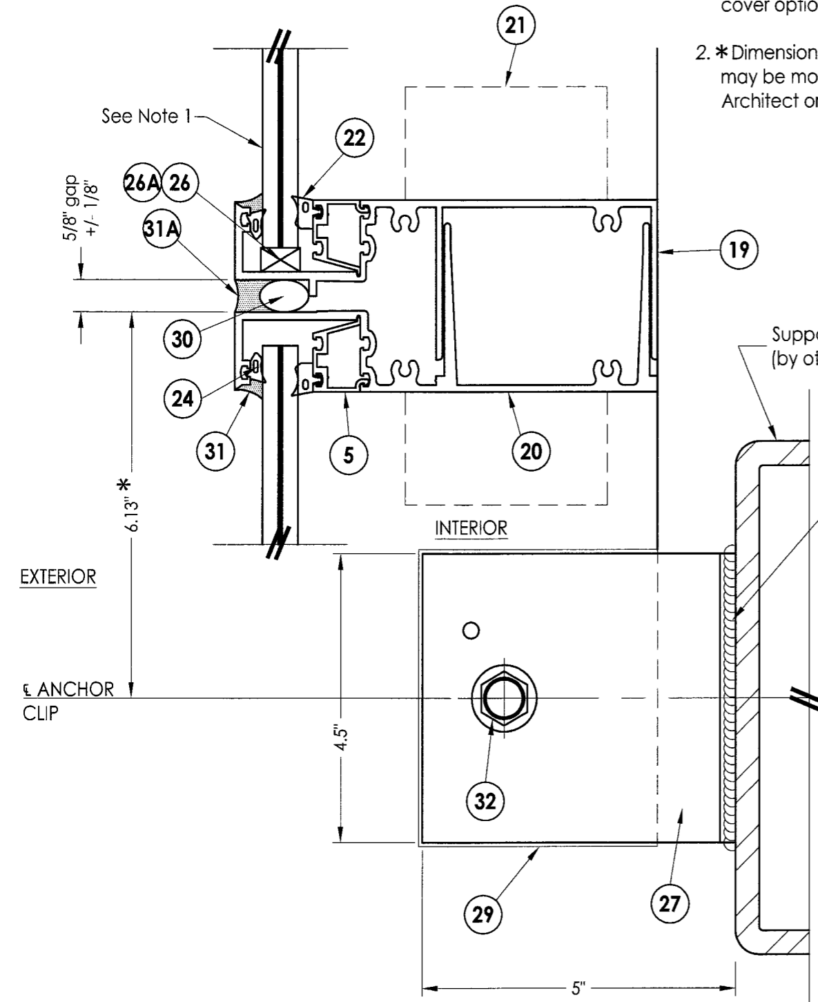
1 VERTICAL CROSS SECTION 8 Intermediate Anchor & Splice Detail
