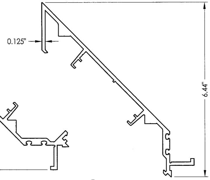
9A FEMALE CORNER
