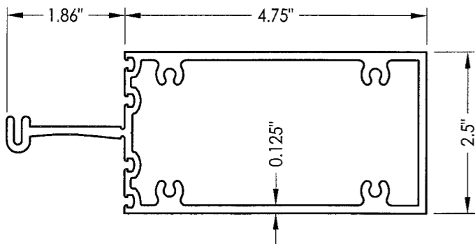
7 INTERMEDIATE HORIZONTAL
