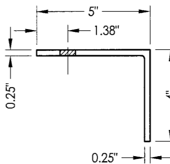
27 DEAD LOAD ANCHOR CLIP
