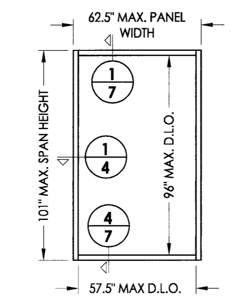
SINGLE PUNCHED OPENING
