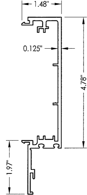
13 MULLION MALE
