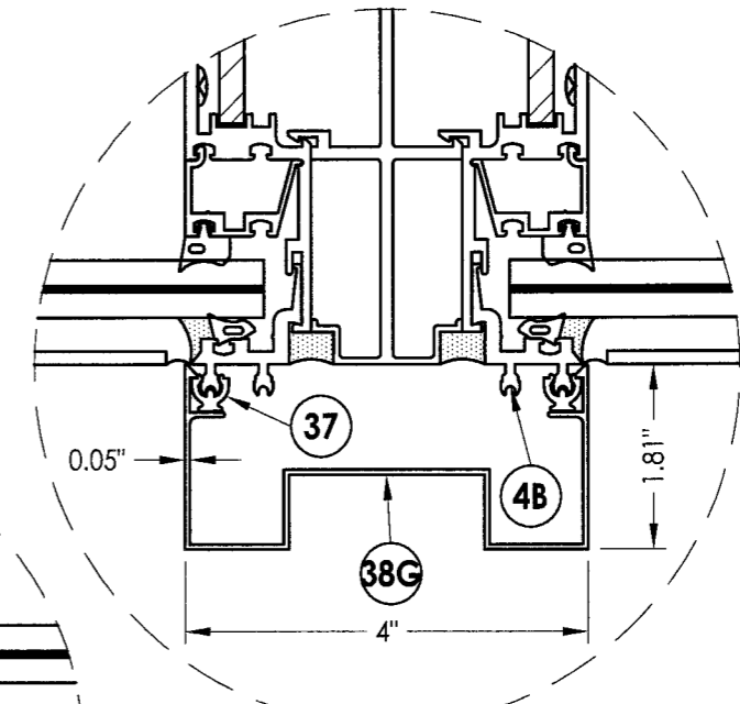
4" NOTCHED VERTICAL FACE COVER
