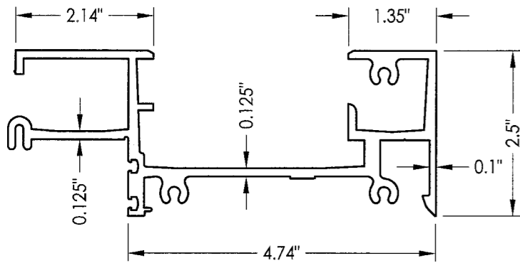
2 HEAD & SILL
