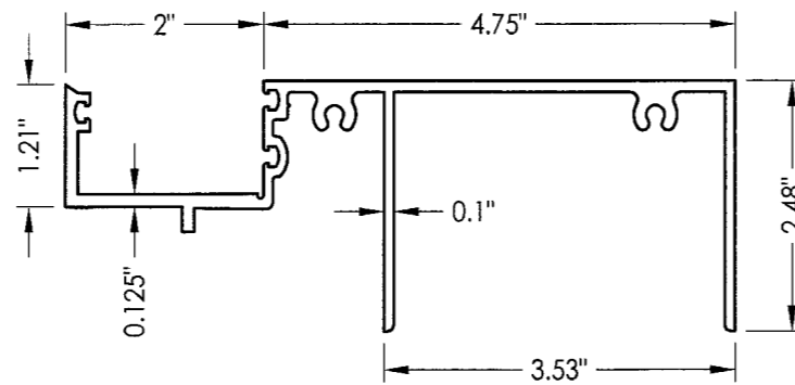
19 TOP TWIN SPAN
