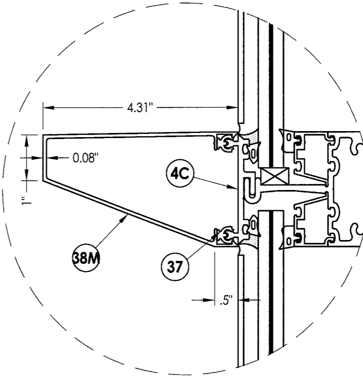
DEEP SLOPED HORIZONTAL FACE COVER OPTION 2
