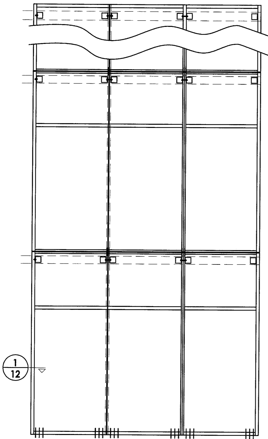
MULTIPLE SPAN FRAME ANCHORING MAX. DP <= 90 PSF (MULTIPLE SPAN)
