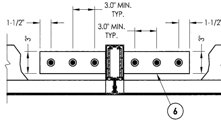
2 12 HORIZONTAL CROSS SECTION @ VERTICAL Sill & sill cover partially removed for clarity Anchor @ head similar
