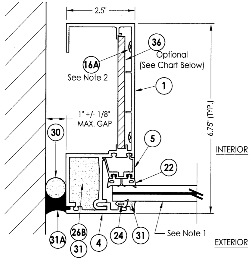
1 HORIZONTAL CROSS SECTION 4 Jamb Detail Dry Glazed Option Total Ix (Aluminum) = 15.189 in. 4
