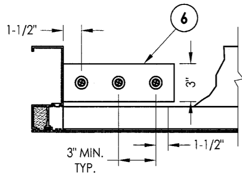
1 12 HORIZONTAL CROSS SECTION @ JAMB Sill & sill cover partially removed for clarity Anchor @ head similar
