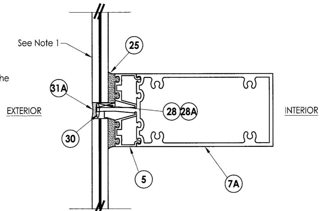
2 VERTICAL CROSS SECTION 8 Intermediate Horizontal Mullion Detail Structural Glazed Option
