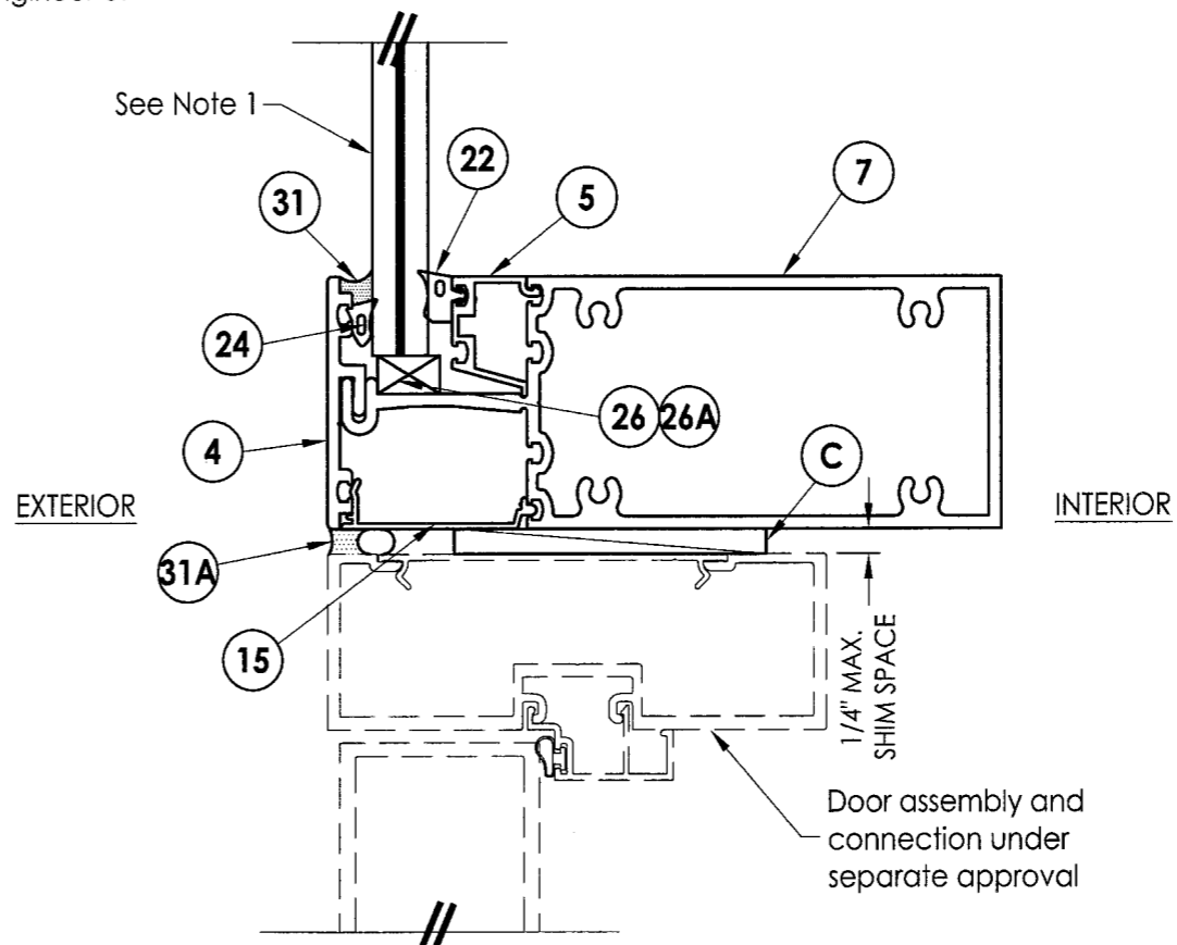
3 VERTICAL CROSS SECTION 8 Intermediate Horizontal Mullion/Door Header Detail
