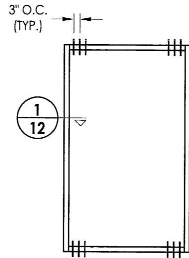
SINGLE PUNCHED OPENING FRAME ANCHORING MAX. DP <= 110 PSF
