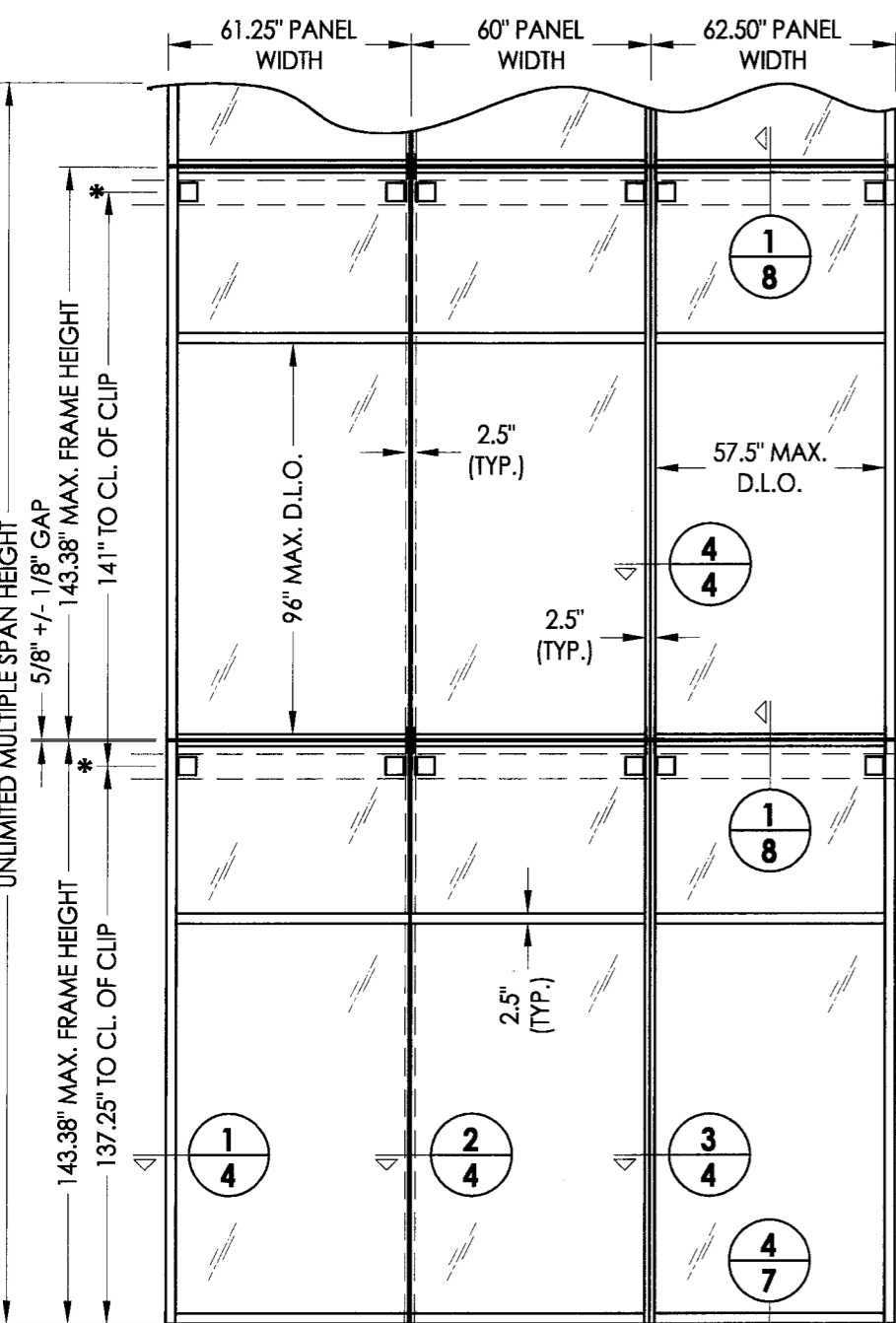
MULTIPLE SPAN
