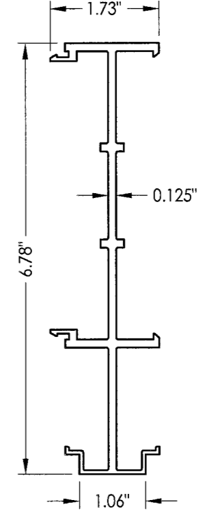
14 MULLION ADAPTOR
