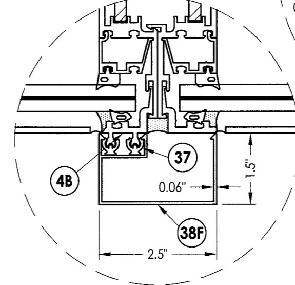
HALF DEEP SQUARE VERTICAL FACE COVER
